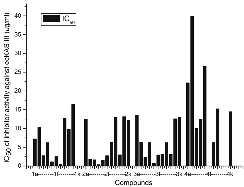
Figure 2. Inhibitory activities of the compounds. IC 50 more than 50 µg/mL not demonstrate.
