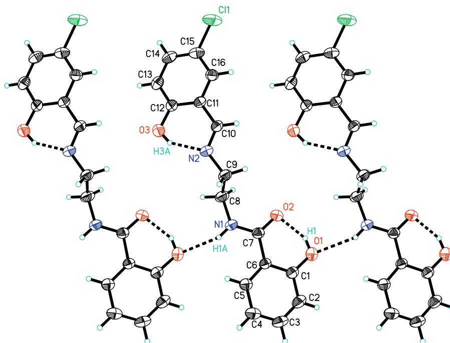
Figure 1. Molecular structure of compound 1c with atoms and hydrogen bonds labeling.
