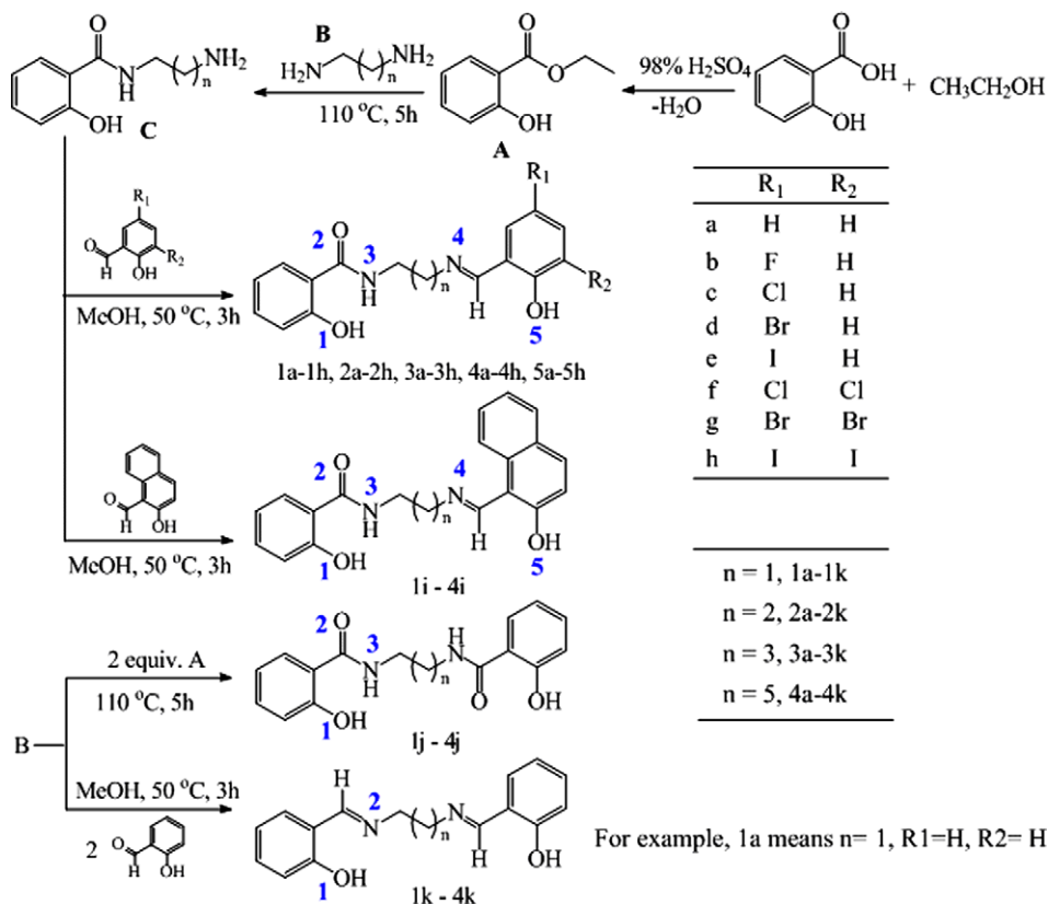
Scheme 1. The general procedure of the synthesized compounds. '1', '2', '3', '4', '5' represent the atom number bonding to the amino acid active site.
