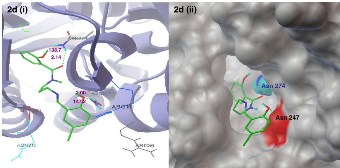
Figure 3. Compound 2d (colored in green) is bound into ecKAS III receptor site via hydrophobic interactions and hydrophilic binding by hydrogen bond between its O2 and H–N of Asn 274 (N–H···O2: 2.14 Å, 138.7°), O5 and H–N of Asn 247 (N–H···O5: 2.00 Å, 147.2°) (2d(i)), and extending into the mouth of the substrate tunnel (2d(ii)).
